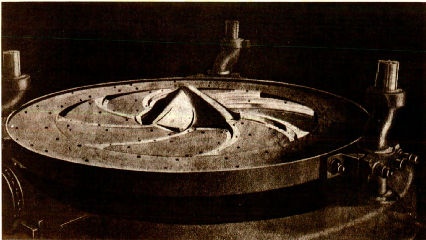
PLATE II—Roller table with M. & S. batters and 'fadeaway' cone
