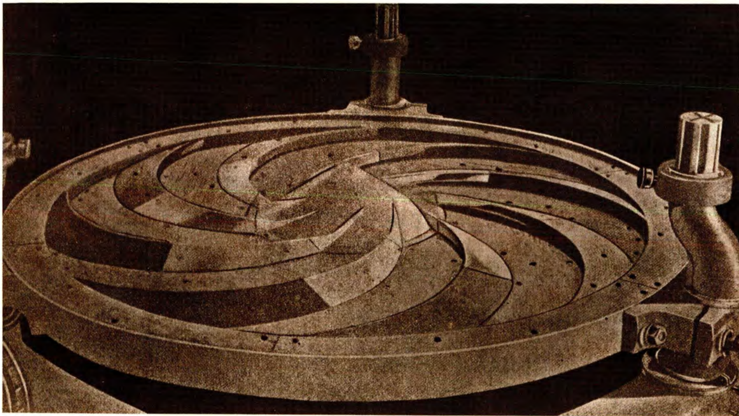
PLATE III—Roller table with Crescent batters and 'fadeaway' cone
